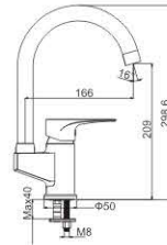
M54323-118C-CI40 Vertical kitchen faucet
