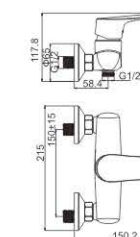
M41372-157LG Shower faucet
