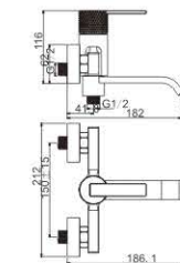
M31633-267LSJ Bath faucet
