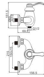
M41025-535C Shower faucet
