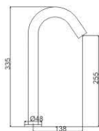
SF11004ZCP-B Sensor faucet
