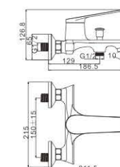
M31585-244C Bath faucet
