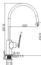
M54513-814C Vertical kitchen faucet
