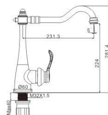
M51264-535H Vertical Kitchen faucet
