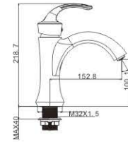
M11434-198RG Basin faucet
