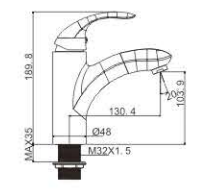
MI4303-121C Basin faucet
