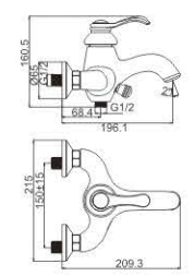
M31025-535C Bath faucet
