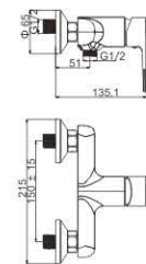
M41534-200C Shower faucet
