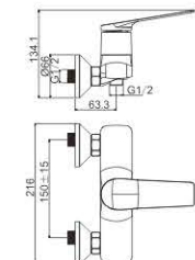
M41585-244C Shower faucet
