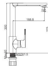
M54441-200C Vertical kitchen faucet
