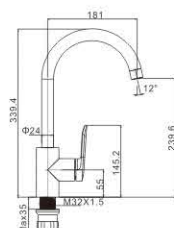
M54570-235H Vertical kitchen faucet
