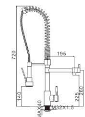
M53318-118C Pull out spray kitchen faucet
