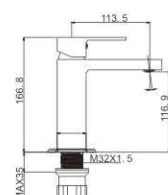
MI1659-273 Basin faucet
