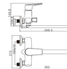
M33372-157LG-S023 Wall bath faucet
