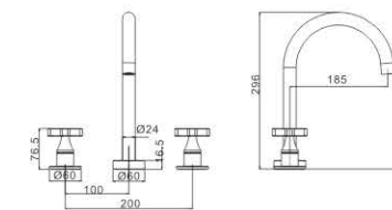
M81686-991C-C589 Bath faucet
