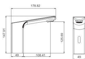
SF11018ZCP-B Sensor faucet
